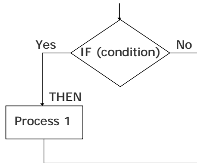
(a) Flowchart
