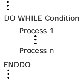
(b) Pseudocode
