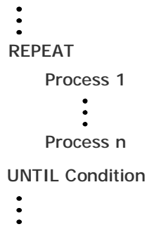
(b) Pseudocode
