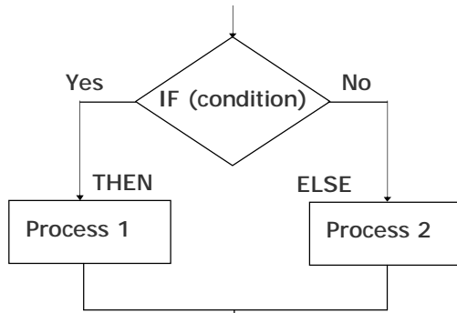
(a) Flowchart
