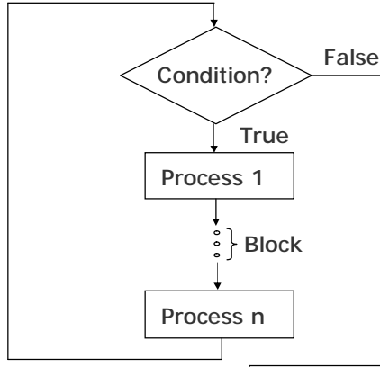
(a) Flowchart
