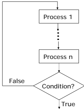
(a) Flowchart
